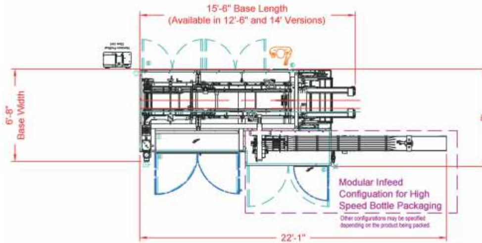
Typical Layout Drawing (Actual conveyor lengths vary by application.)
