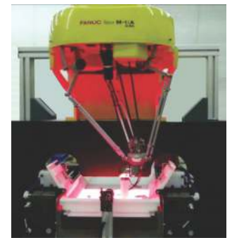
Flex Feeder with M-1iA Robot
