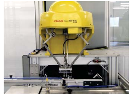
Robotic Infeed for Diagnostic Test Kit to Pouching Machine
