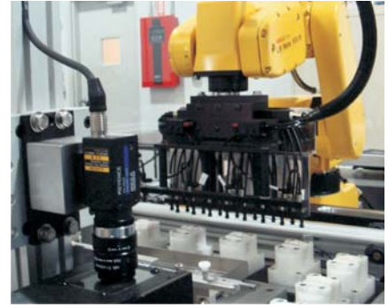
Vision Inspection Camera for Diagnostic Test Kits
