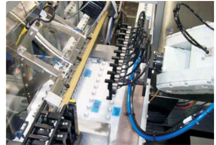
End Effector for Robotic Assembly of Drug Delivery Device
