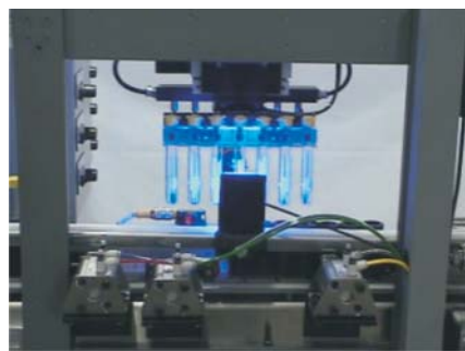
Diagnostic Test Kit Inspection Station
